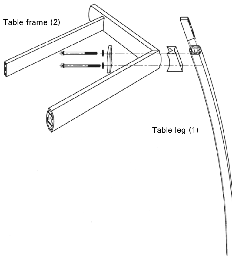
Allen screw, M8 x 110 (7) 4 pieces
